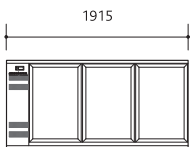
Remote front elevation
