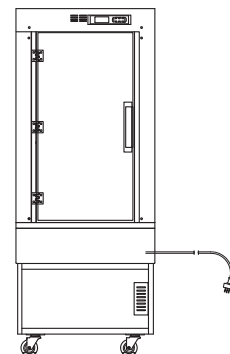
REAR VIEW
