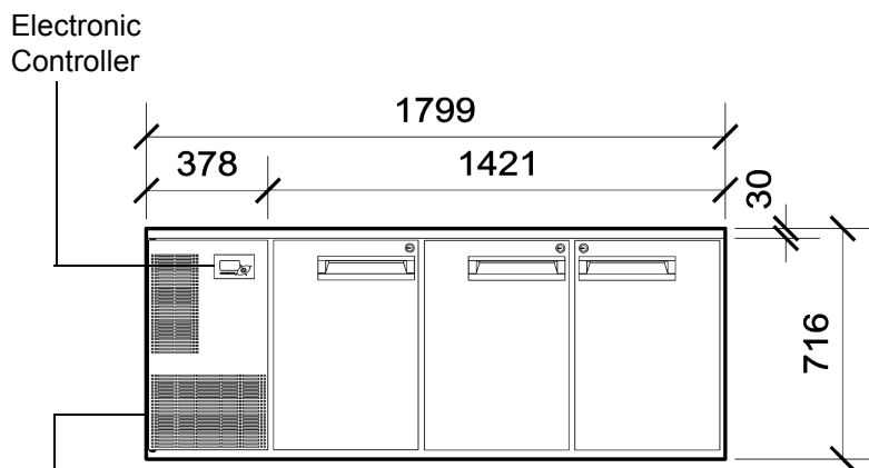
Side Mounted Integral Refrigeration Unit
