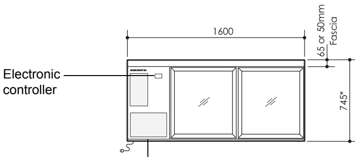
Side mounted integral refrigeration unit
