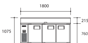
Integral front elevation
