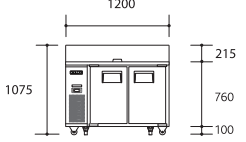
Integral front elevation
