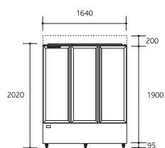
Integral/remote front elevation
