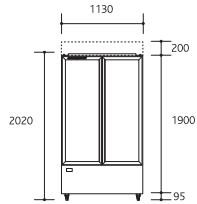
Integral/remote front elevation
