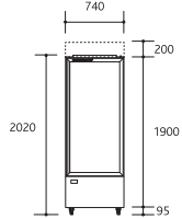
Integral/remote front elevation
