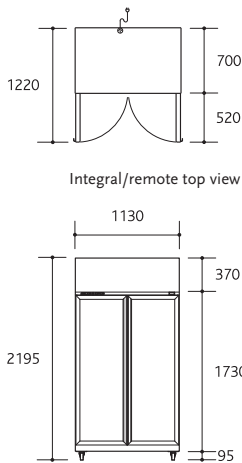
Integral/remote front elevation
