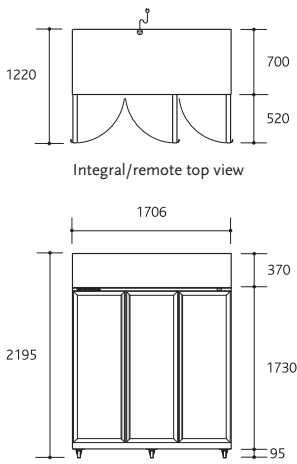
Integral/remote front elevation
