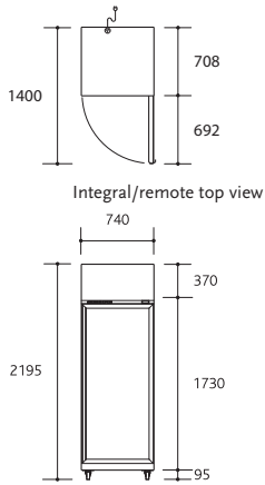
Integral/remote front elevation
