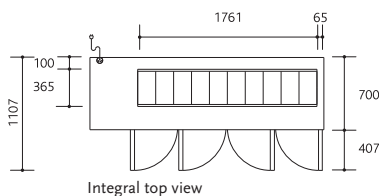
Integral top view
