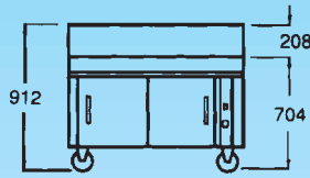
WORKING SIDE ELEVATION WDB/HC MODELS
