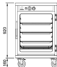
Front Elevation
